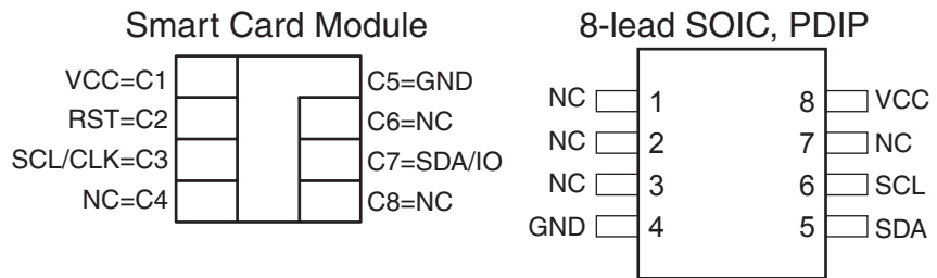
Figure 1. Package Options
